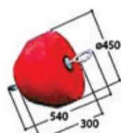
UB-30 Volum 30 liter Art. no 3267012/17/18 Vekt 6,0 kg
