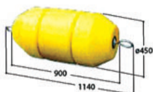
UB-110 Volum 110 liter Art. no 3267032/37/38 Vekt 14,0 kg
